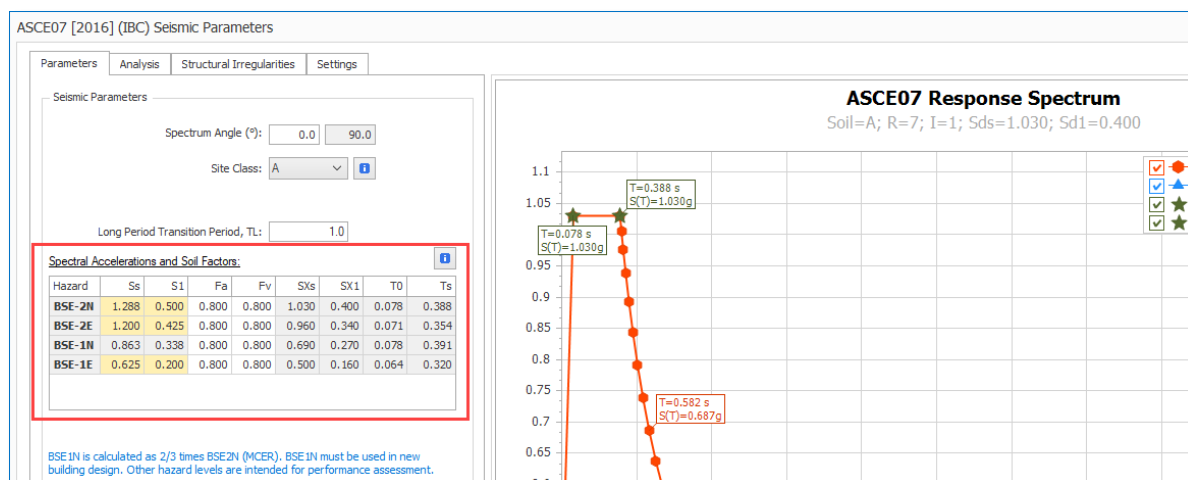
ASCE07 Seismic parameters UI in ProtaStructure for seismic hazard definition.
